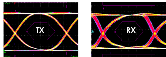
1.25 Gb/s, 2 -1 NRZ Data Eye pattern
