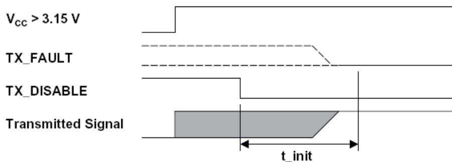
Power on initialization of SFP, TX_DISABLE asserted Initialization during hot plugging of SFP TRANSCEIVER
