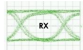
4.25 Gb/s, 2 23 -1 NRZ Data Eye Pattern
