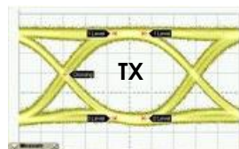
4.25 Gb/s, 2 23 -1 NRZ Data Eye Pattern
